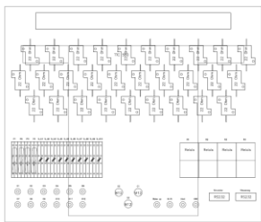
Hardware-Simulation der Hydraulik Ventile
